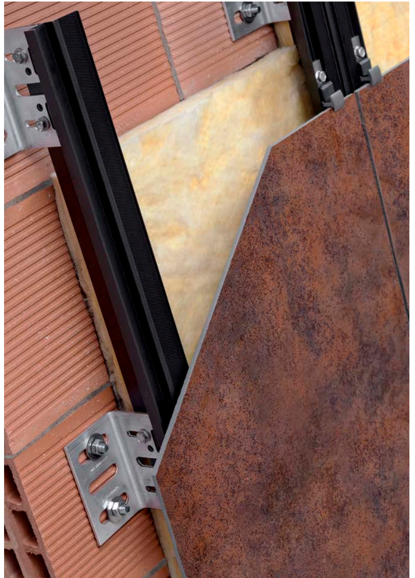
Image 27: VM System detail
