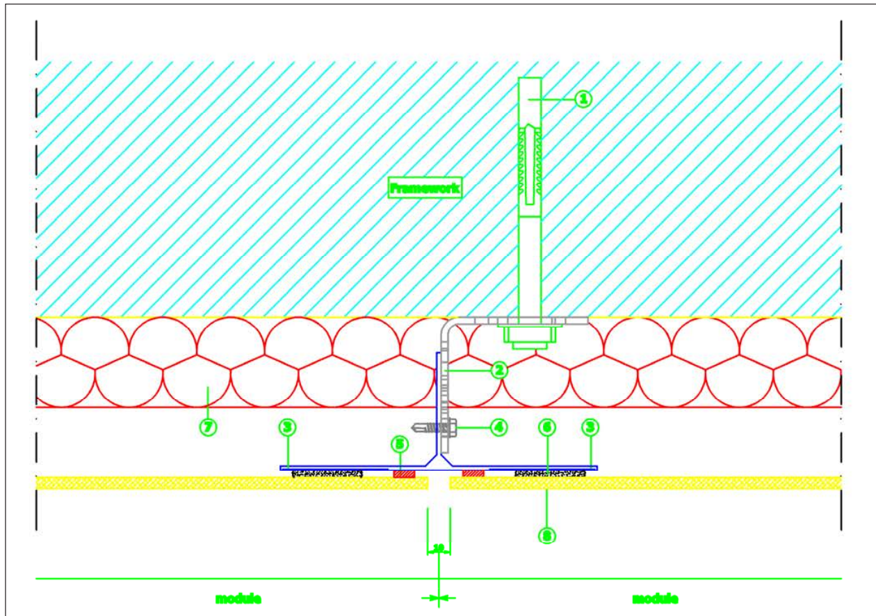
Image 13: Expansion joint on HC System
