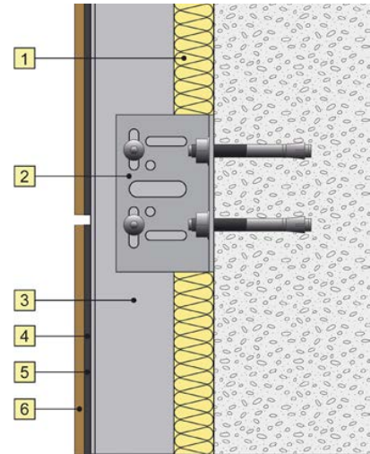
Image 16: HC System vertical section
