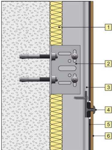
Image 26: VM System vertical section
