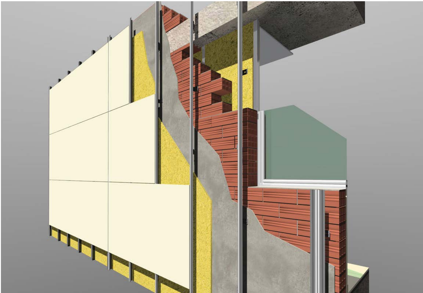
Image 15: HC System mockup
