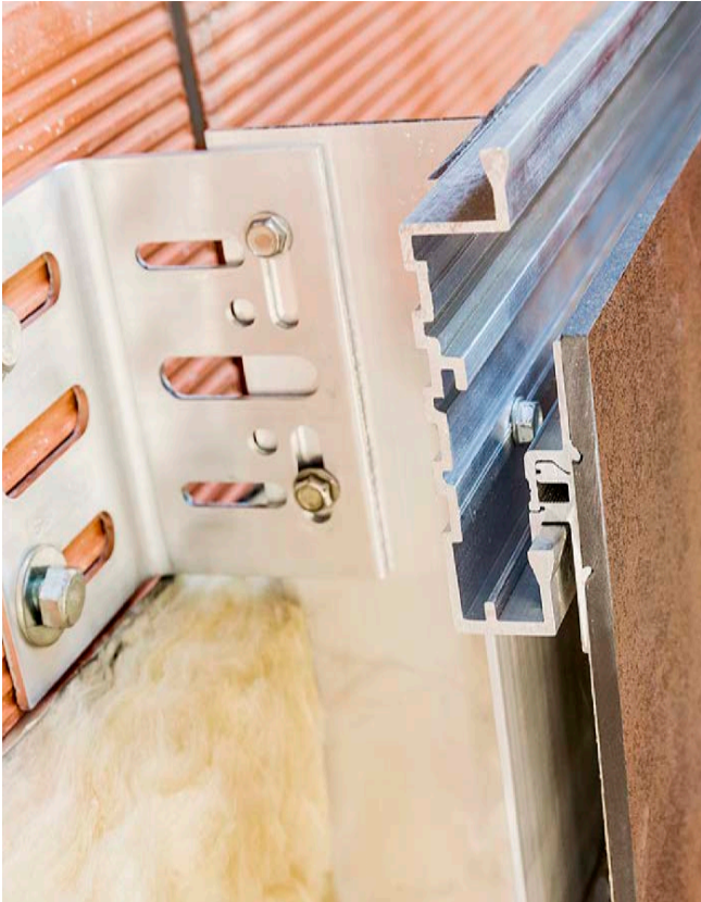
Image 40: Strongfix System details
