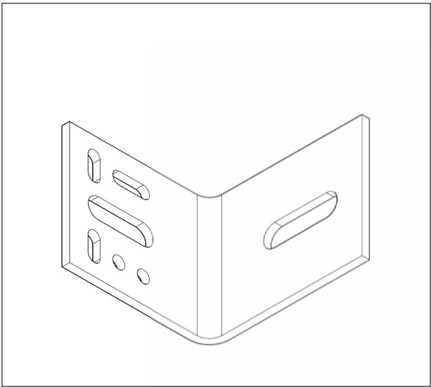
Image 22: Suporting bracket
