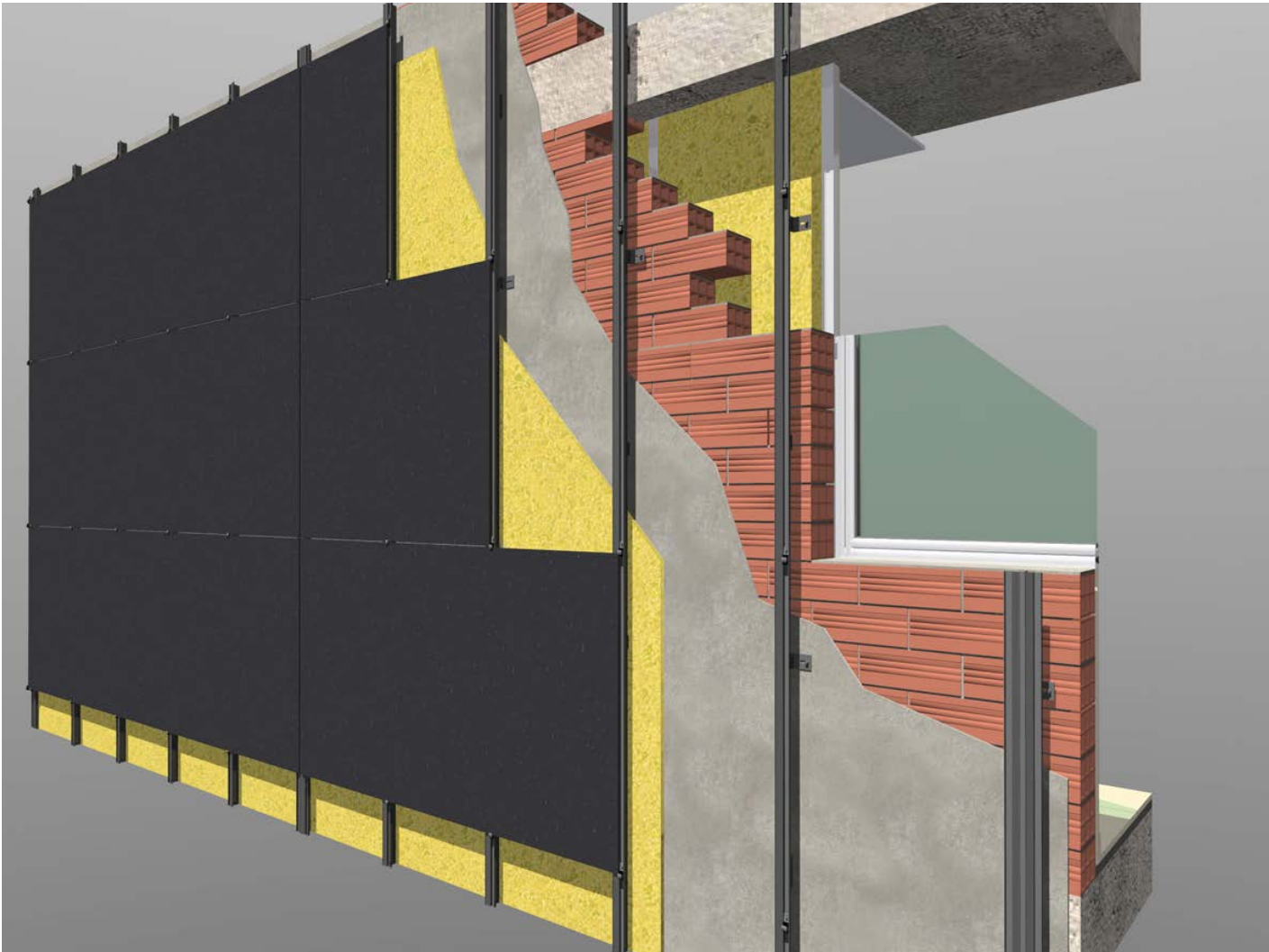
Image 25: VM System mockup
