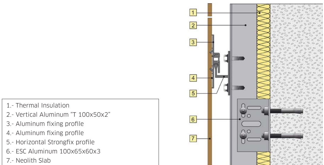
Image 38: Strongfix System vertical section
