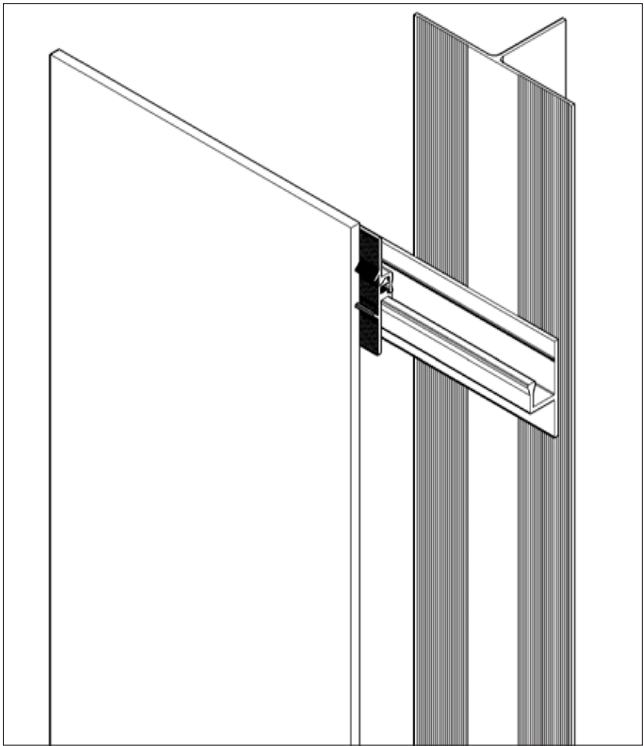
Image 48: Strongfix System detail
