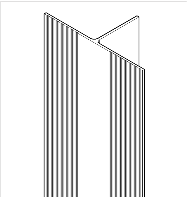
Image 24: Vertical profile
