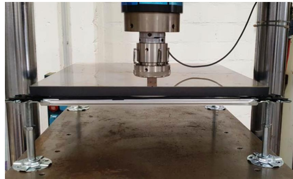
Fig 24 Testing raised flooring with VETRITE
